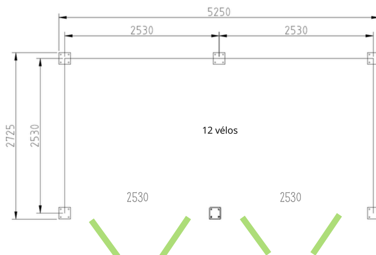
Abri Jungle Compact 5m x 2,5m
