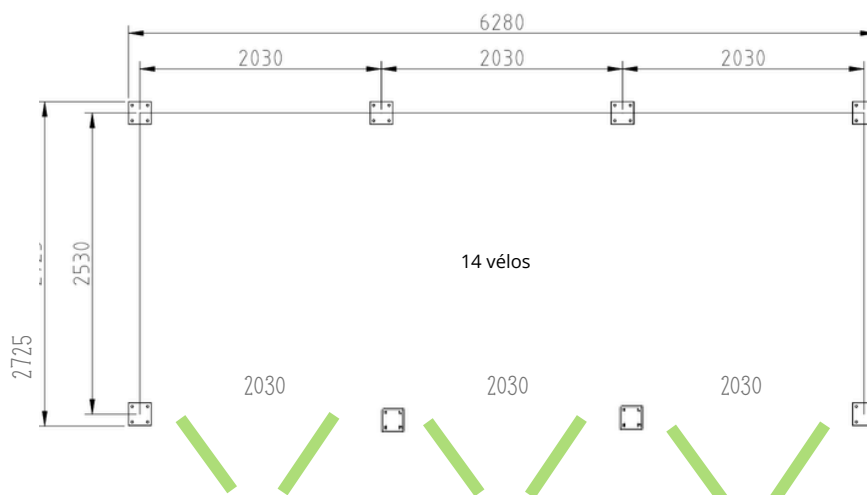
Abri Jungle Compact 6m x 2,5m
