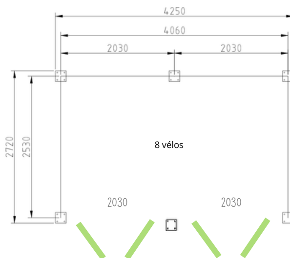
Abri Jungle Compact 4m x 2,5m
