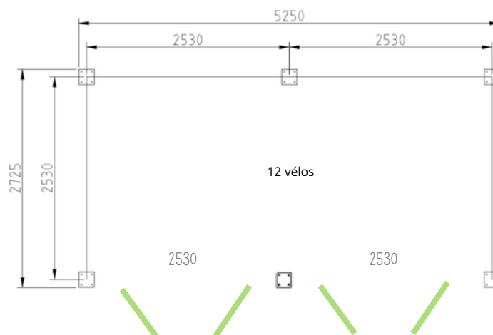
Abri cyclage Compact 5m x 2,5m
