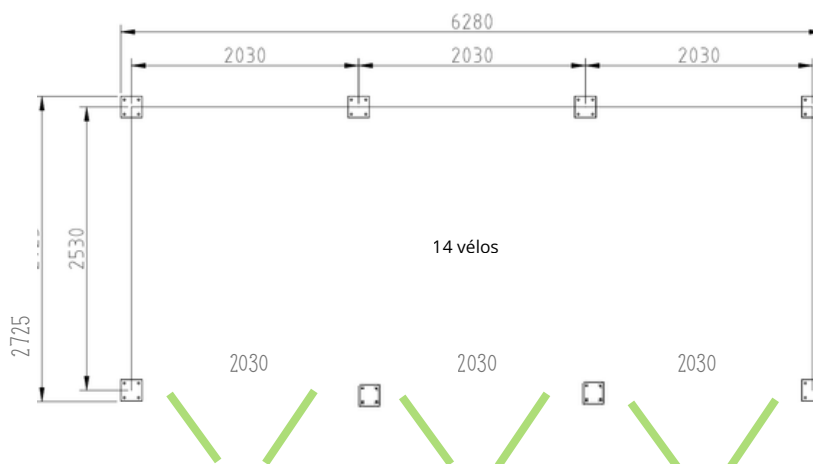
Abri cyclage Compact 6m x 2,5m
