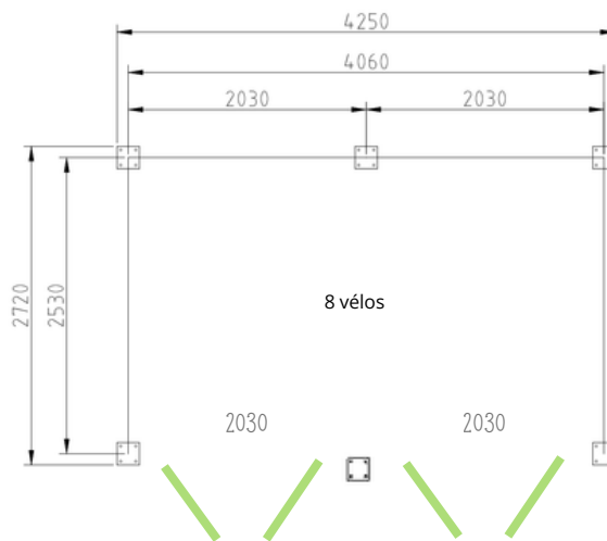
Abri Cyclage Compact 4m x 2,5m
