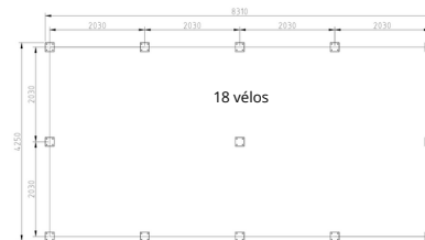
Abri Forêt 8m x 4m
