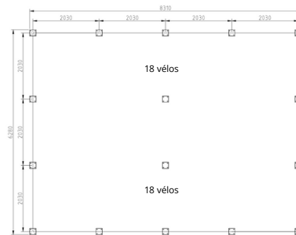
Abri Forêt 8m x 6m
