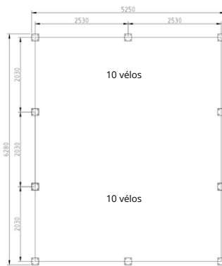
Abri Refuge 5m x 6m
