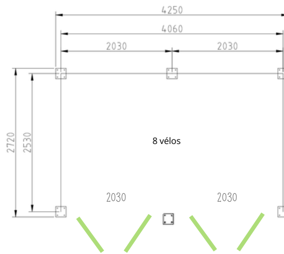
Abri rachais Compact 4m x 2,5m
