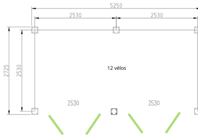
Abri rachais Compact 5m x 2,5m
