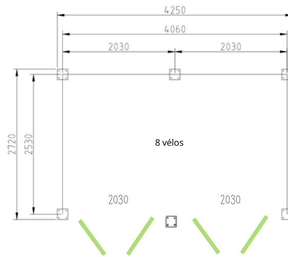
Abri lapiaz Compact 4m x 2,5m
