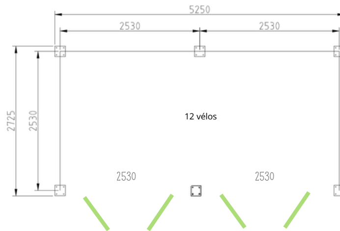
Abri lapiaz Compact 5m x 2,5m
